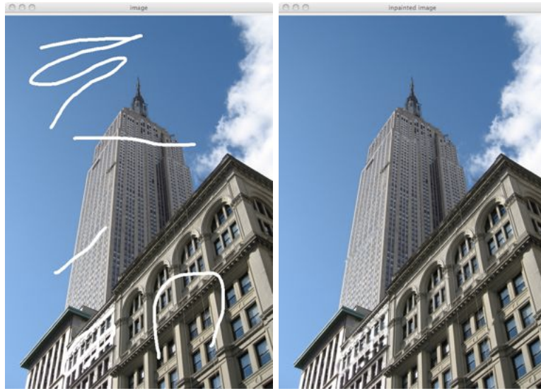
Figure 10.8: An example of inpainting with OpenCV. The left image shows areas marked by a user as "corrupt". The right image shows the result after inpainting.
